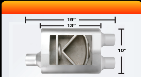
4"x10"x13" OFFSET/DUAL
