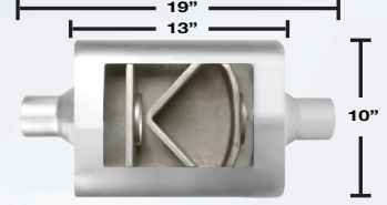
4"x10"x13" CENTER/CENTER
