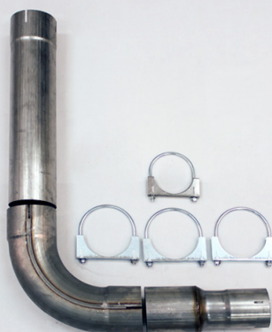
409 STAINLESS DIESEL SINGLE EXHAUST STACK KIT
