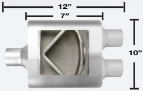
4"x10"x7" CENTER/DUAL
